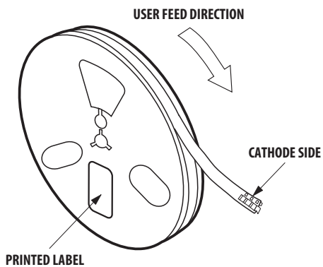
Figure 9. Reeling Orientation
