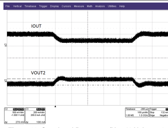
Figure 22. Step Load Response ( V_{IN}=48 V , I_{OUT1}=0 , Step Load on I_{OUT2}=100 mA to 200 mA)
