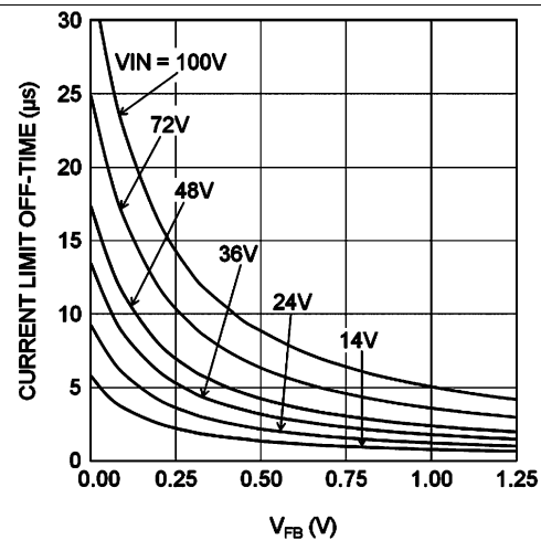
Figure 6. T_{ON} (I_{LIM}) vs V_{FB} and V_{IN}
