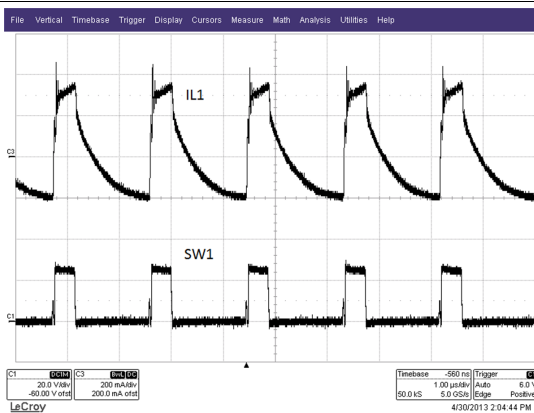
Figure 21. Steady State Waveform ( V_{IN}=48 V , I_{OUT1}=100 mA, I_{OUT2}=200 mA)
