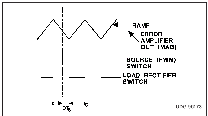
Figure 3. Circuit waveforms.
