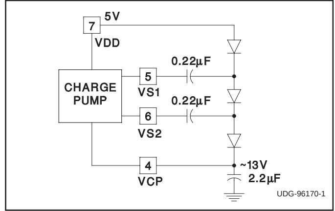
Figure 9. Charge pump circuits.
