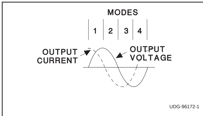
Figure 2. Operating modes.
