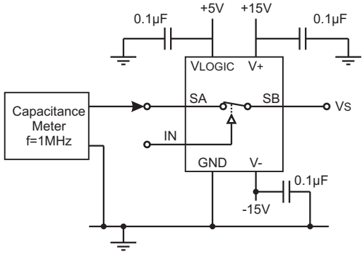
Figure 9 - On Capacitance
