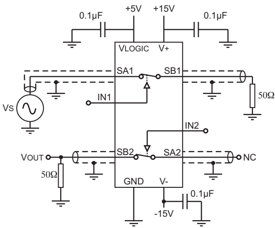
Figure 7 - Channel-to-Channel Crosstalk
