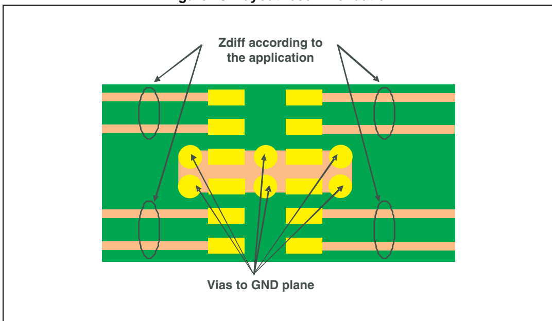
Figure 20. Layout recommendation
