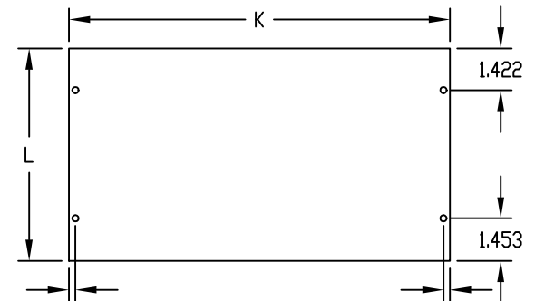
REAR PANEL
