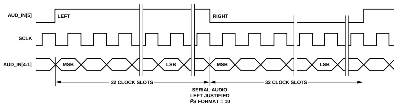
Figure 26. Serial Audio—Left-Justified
