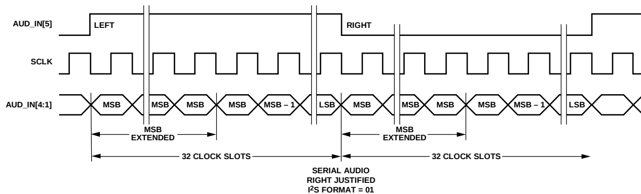
Figure 25. Serial Audio—Right-Justified
