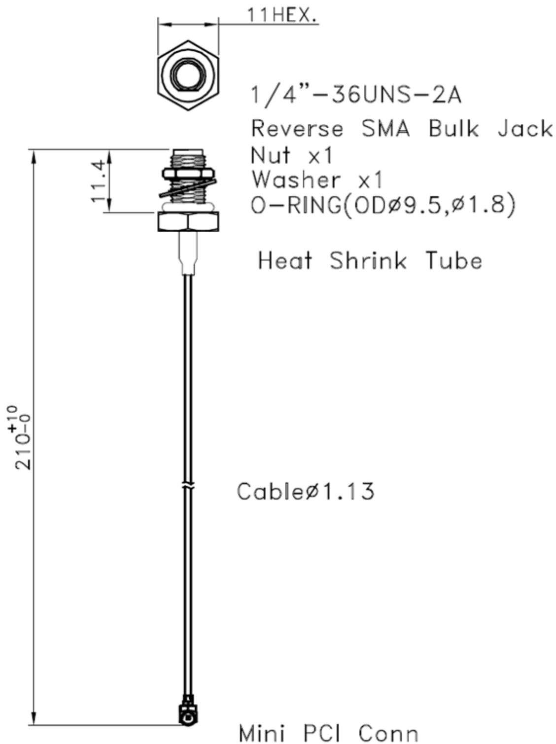
Figure 1 Physical Dimensions
