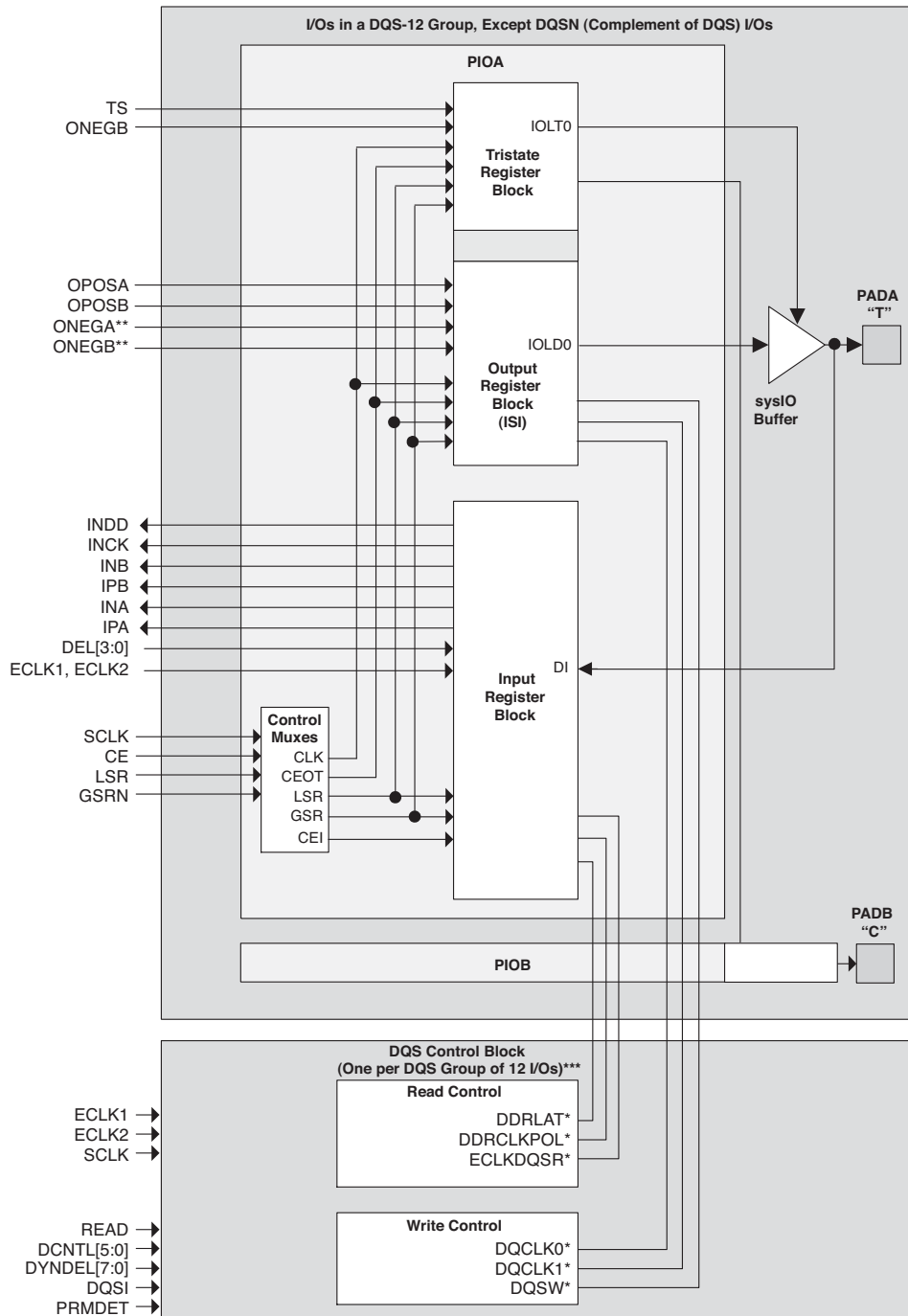
Figure 2-31. PIC Diagram
