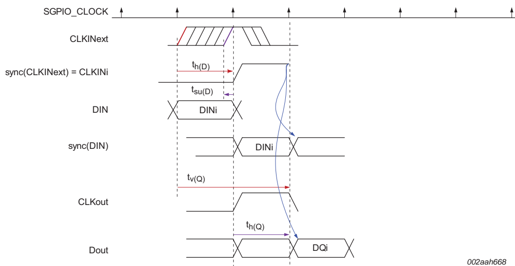
Fig 30. SGPIO timing
