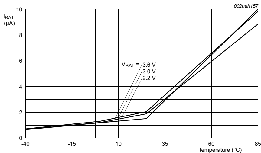
Fig 16. Typical battery supply current versus temperature in Deep power-down mode
