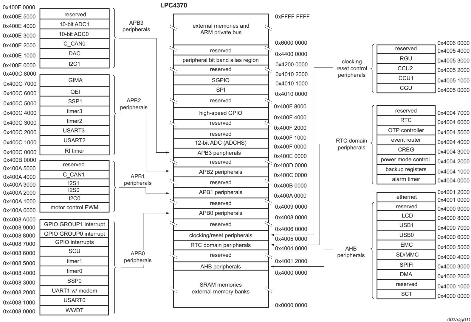
Fig 6. LPC4370 Memory mapping (peripherals)
