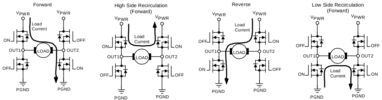
Figure 12. 34932 Power Stage Operation
