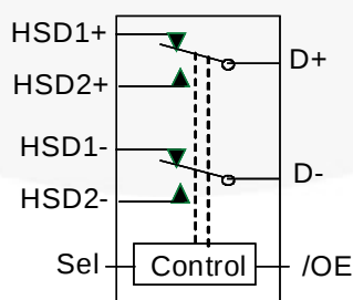
Figure 1. Analog Symbol
