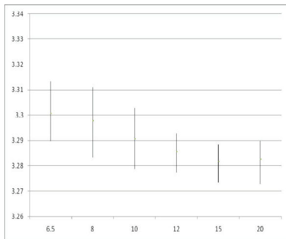
Fig. 14: Line Load Regulation 3.3V
