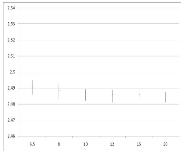
Fig. 15: Line Load Regulation 2.5V
