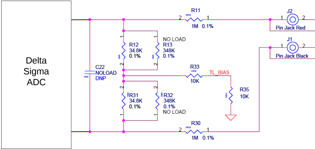
Figure 3-2. Circuit Diagram
