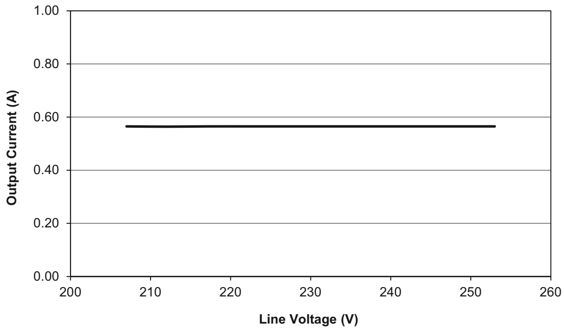
Figure 14. Output Current vs. Line Voltage
