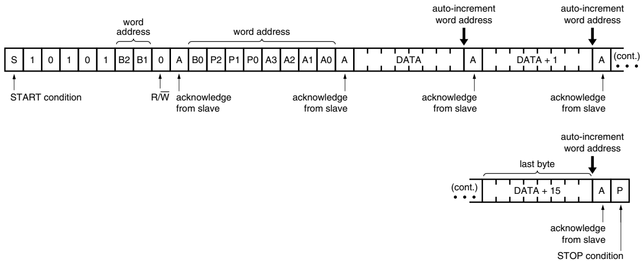
Fig 7. Page write operation (16 bytes)
