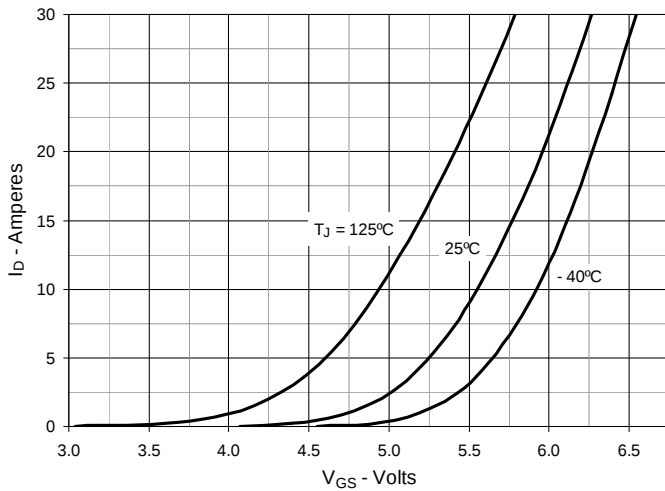
Fig. 7. Input Admittance
