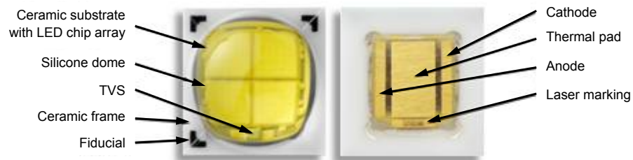
Figure 3. Pad configuration.
