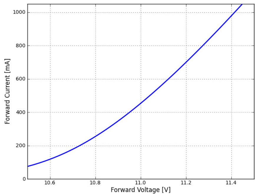
Figure 13. Forward current vs. forward voltage (12V).
