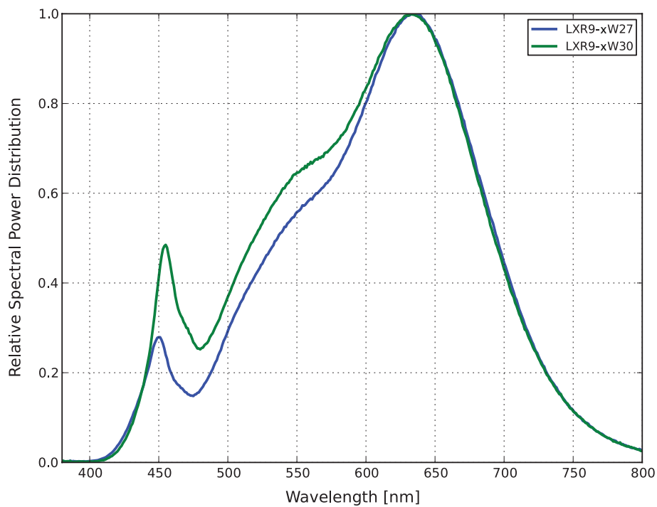
Figure 7. Color spectrum of LXR9-xWxx emitter, integrated measurement.
