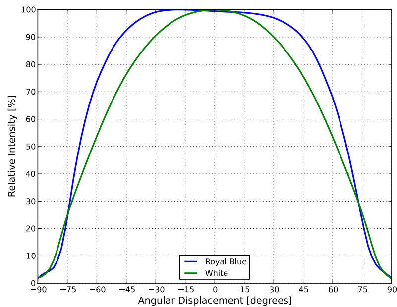
Figure 16. Typical representative spatial radiation pattern.
