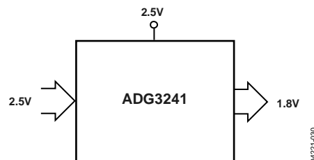
Figure 30. 2.5 V to 1.8 V Voltage Translation, \overline{SEL} = 2.5 V CC
