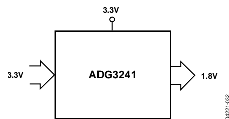
Figure 32. 3.3 V to 1.8 V Voltage Translation, \overline{SEL} = 0 V
