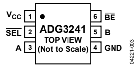
Figure 3. 6-Lead SOT-66
