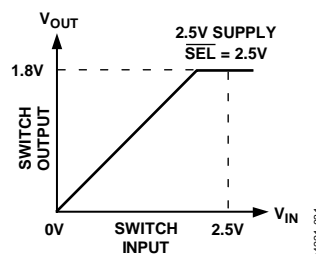
Figure 31. 2.5 V to 1.8 V Voltage Translation, \overline{SEL} = V_{CC}
