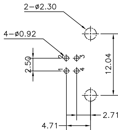
USB-PCB LAYOUT
