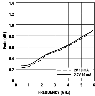
Figure 17. Fmin vs. Bias over Frequency [2] .
