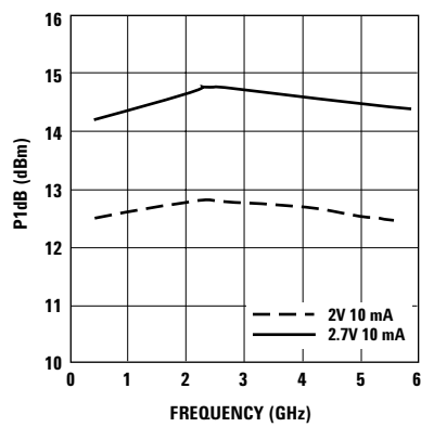
Figure 20. P1dB vs. Bias over Frequency [1] .
