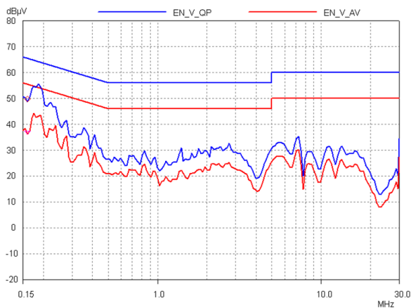
Figure 51 – 115 VAC, Neutral.
