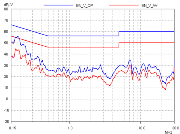
Figure 50 – 115 VAC, Line.
