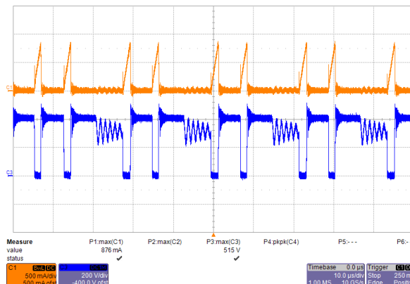
Figure 19 – 230 VAC, Full Load.
