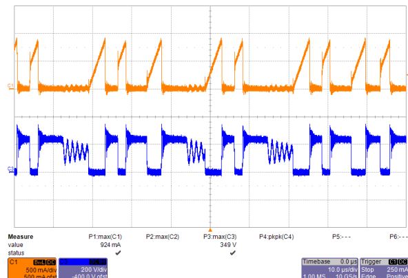
Figure 18 – 115 VAC, Full Load.
