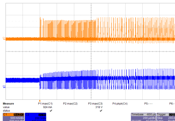
Figure 21 – Start-up Profile, 90 VAC, Full Load
