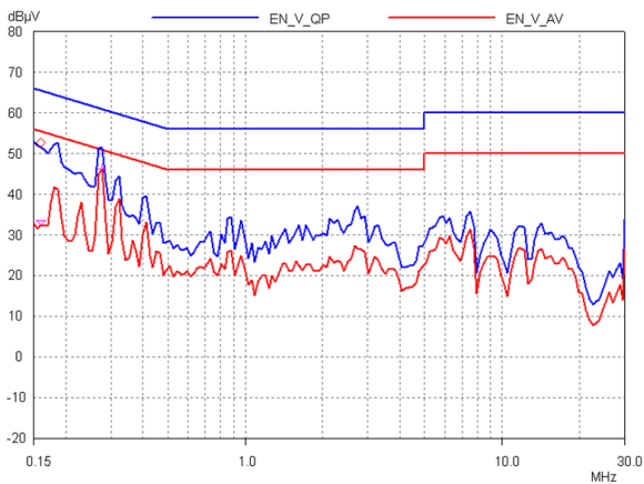
Figure 53 – 230 VAC, Neutral.
