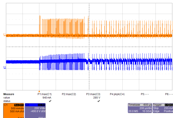
Figure 20 – Start-up Profile, 90 VAC, No-Load
