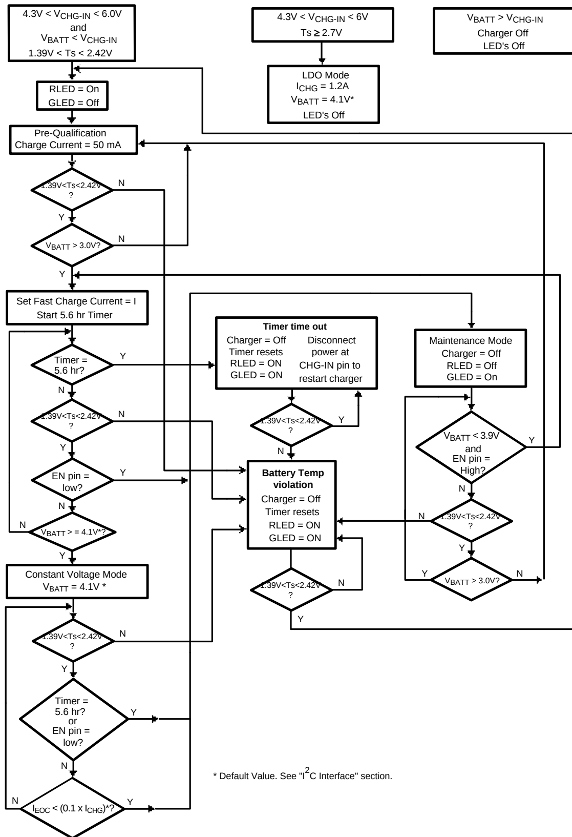
Figure 4. LP3947 Charger Flow Chart
