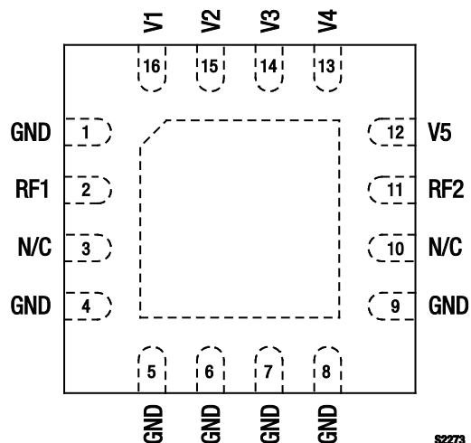
Figure 2. SKY12328-350LF Pinout – 16-Pin QFN (Top View)
