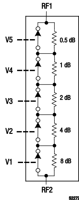
Figure 1. SKY12328-350LF Block Diagram
