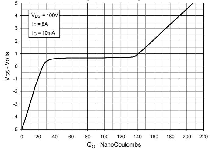
Fig. 14. Gate Charge
