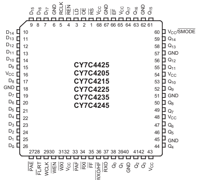
Figure 2. PLCC (Top View)
