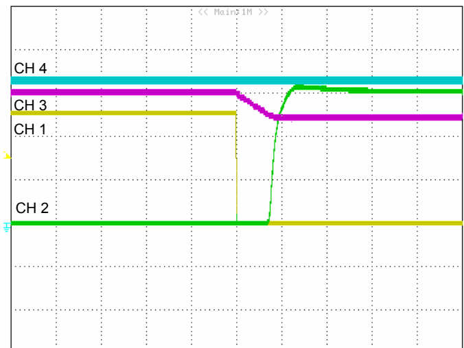
Figure 4: Oring for one feed loss (500uS/div): CH1: linA (2A/div) CH2: linB (2A/div). CH3: VRTN_OUT reference to -48V_OUT (10V/div). CH4: VMGMT_PWR (1V/div).
