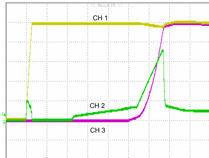
Figure 3: Inrush current (2mS/div): CH1: Vin (VRTN_AF reference to -48V_AF, 10V/div). CH2: lin (-48V_AF, 2A/div). CH3: VRTN_OUT reference to -48V_OUT (10V/div).
