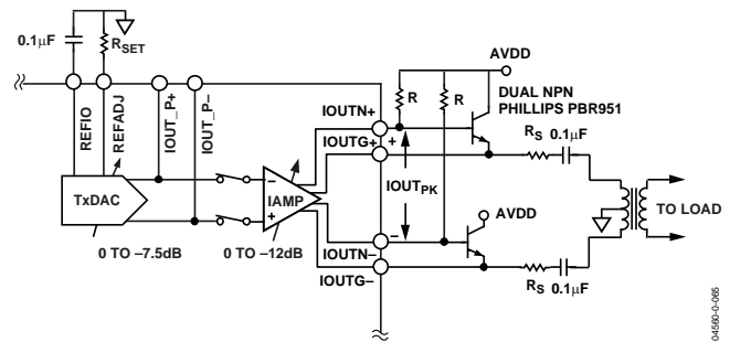
Figure 65. Voltage-Mode Operation
