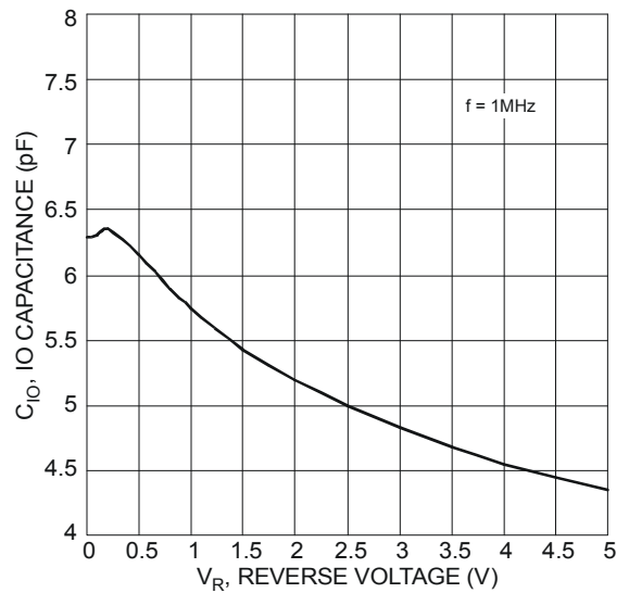
Figure 8 Typical Junction Capacitance
