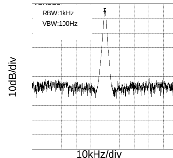
Fig.3 54MHz spectrum (VDD=3.3V,CL=15pF,Ta=25°C)
