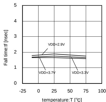
Fig.61 54MHz Fall-time temperature characteristics
