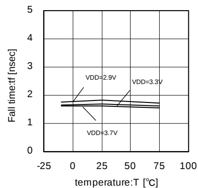
Fig.66 67.5MHz
