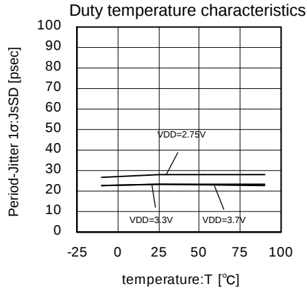
Fig.82 48MHz Period-Jitter 1σ temperature characteristics
