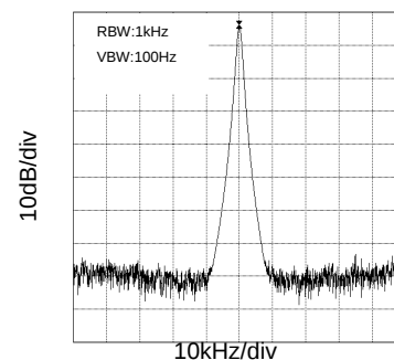
Fig.6 27MHz spectrum (VDD=3.3V,CL=15pF,Ta=25°C)
