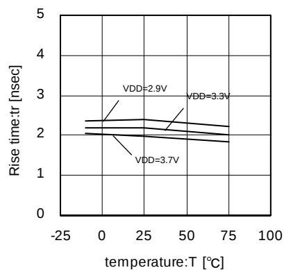
Fig.65 67.5MHz
