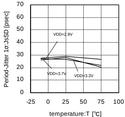
Fig.67 67.5MHz Period-Jitter 1σ temperature characteristics
