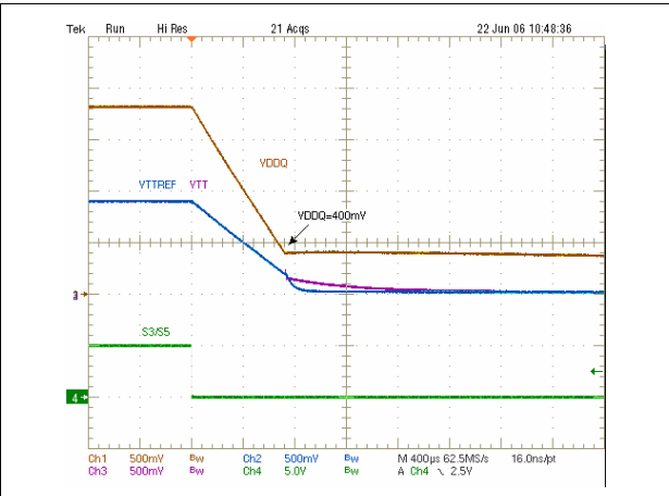
Figure 20. Tracking (fast) discharge, LDOIN = VDDQ
