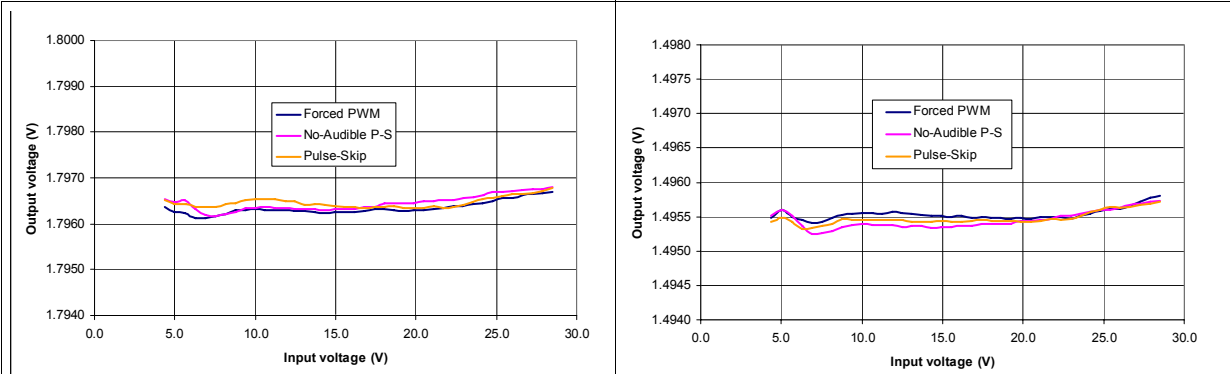
Figure 7. VDDQ line regulation, 1.8 V, 7 A Figure 8. VDDQ line regulation, 1.5 V, 7 A
