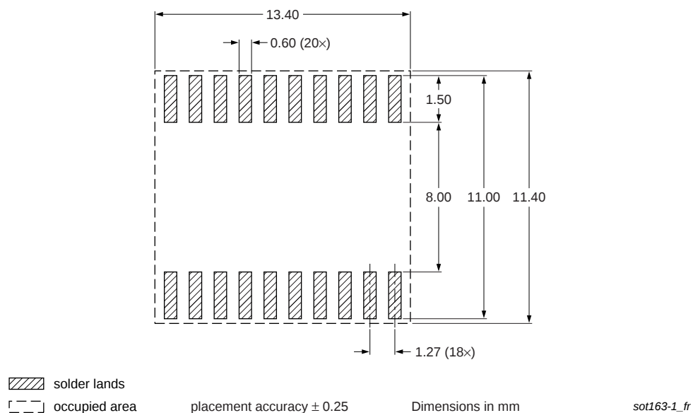
Fig 46. Footprint information for reflow soldering of SO20 package
