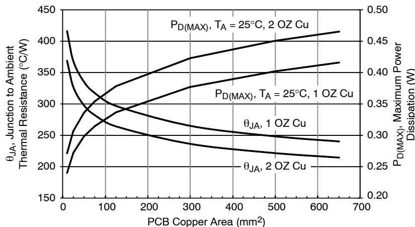
Figure 50. \theta_{JA} and P_{D(\text{MAX})} vs. Copper Area (TSOP-5)
