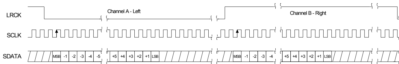
Figure 4. Format 1, 24-Bit Data I²S
