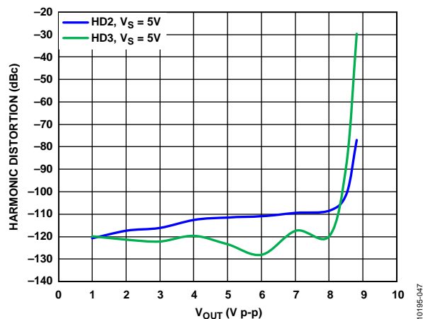
Figure 40. Harmonic Distortion vs. V_{OUT,DM} , f = 10 kHz
