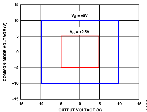
Figure 8. Input Common-Mode Voltage vs. Output Voltage, V_S = \pm 5\text{ V} and \pm 2.5\text{ V}
