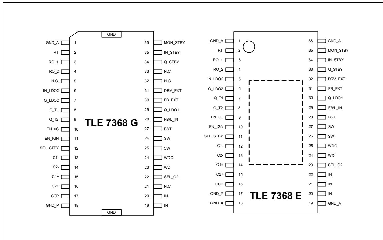
Figure 2 Pin Configuration
