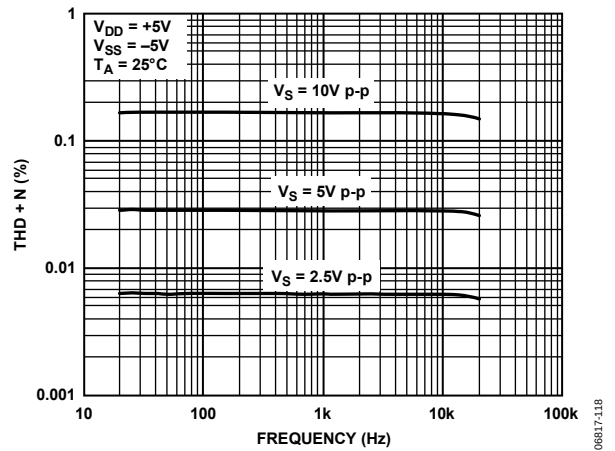
Figure 22. THD + N vs. Frequency, 5 V Dual Supply
