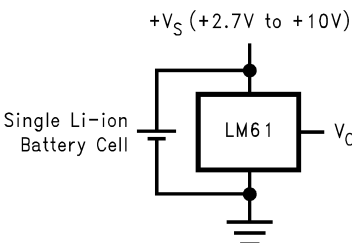
Figure 1. Full-Range Centigrade Temperature Sensor (–30°C to +100°C) Operating from a Single Li-Ion Battery Cell
