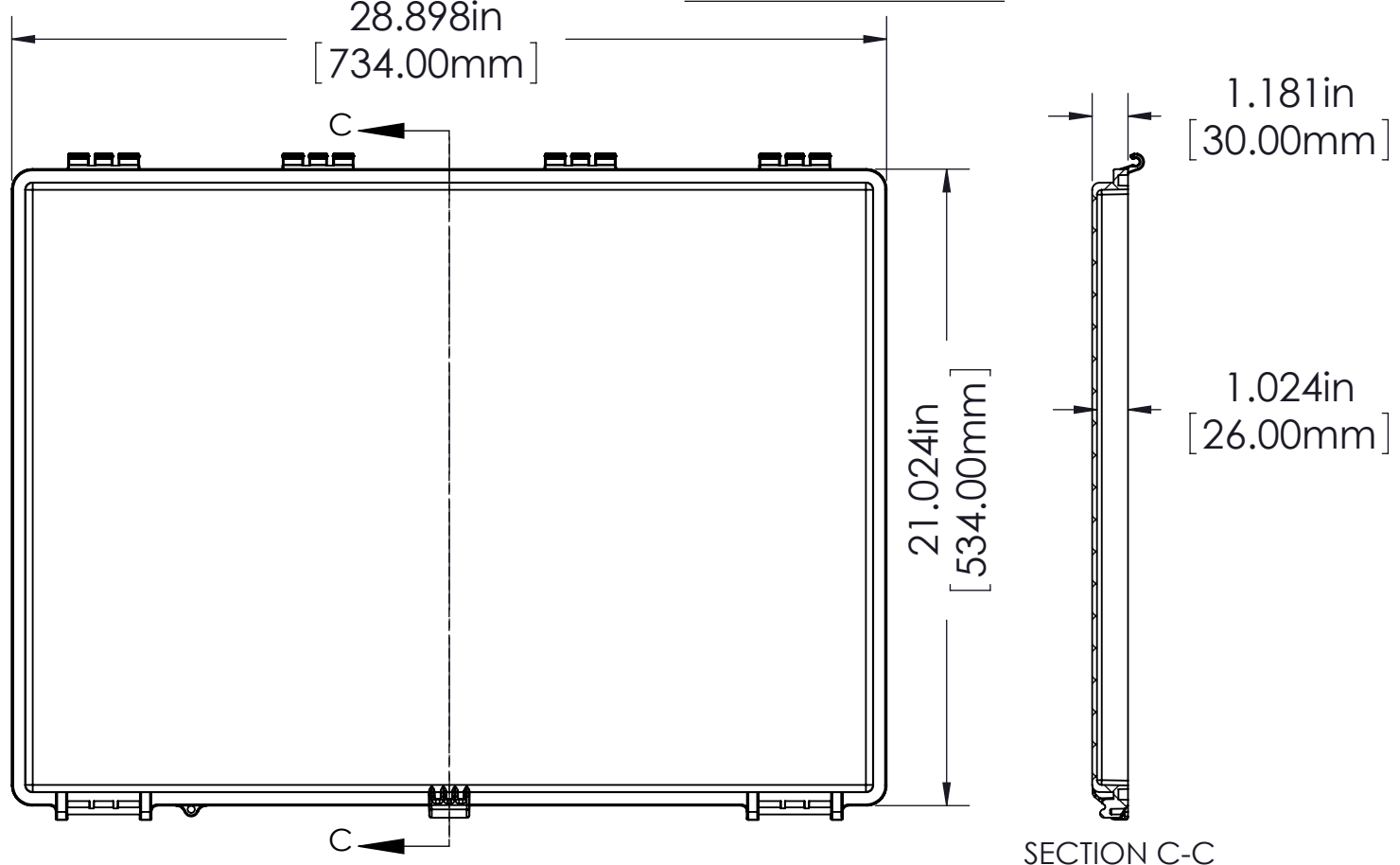
SECTION C-C
