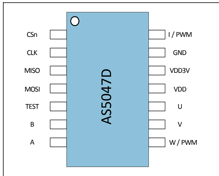
Figure 3: TSSOP-14 Pin Assignment
