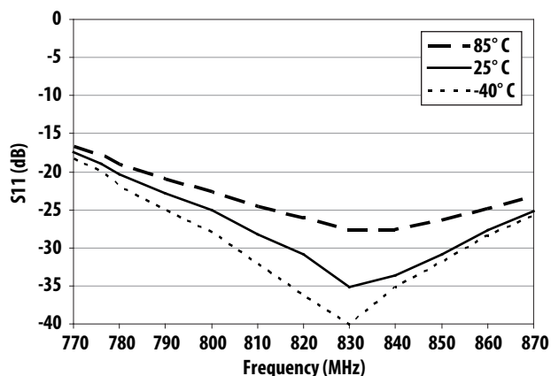
Figure 11. S11 vs Frequency
