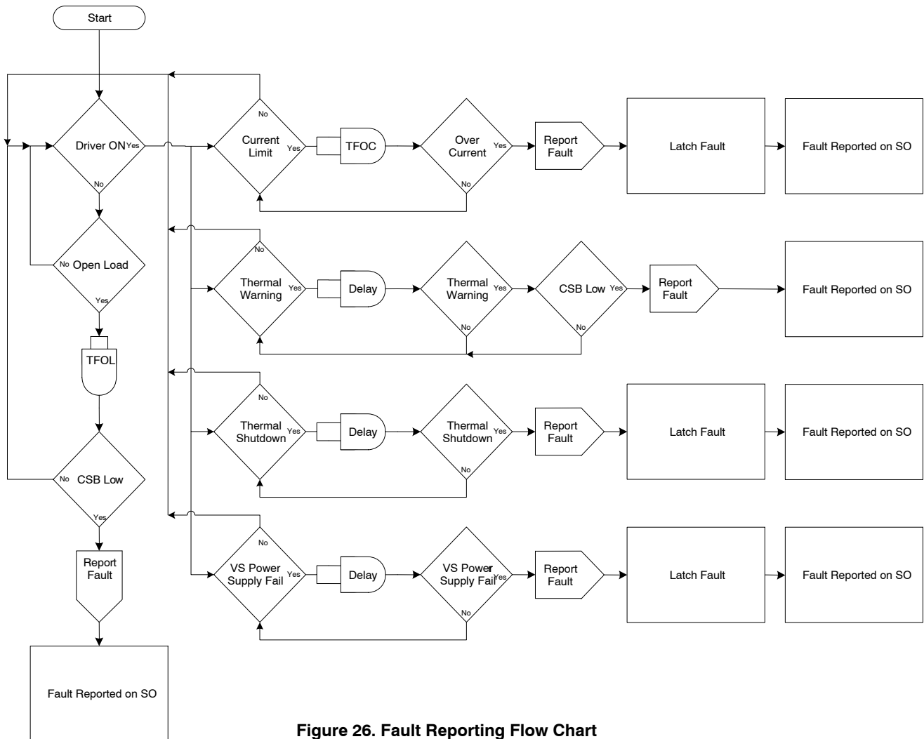
Figure 26. Fault Reporting Flow Chart
