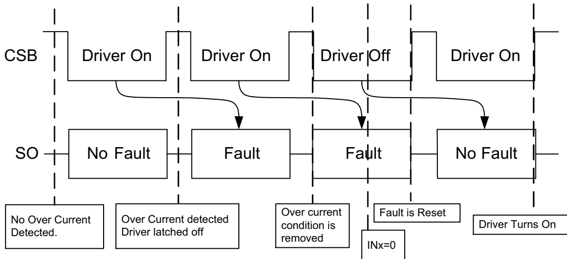
Figure 32. Over Current Timing Diagram
