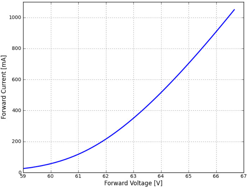
Figure 18. Forward current vs. forward voltage for LXXKx-Pxxx-xx24(A) products.
