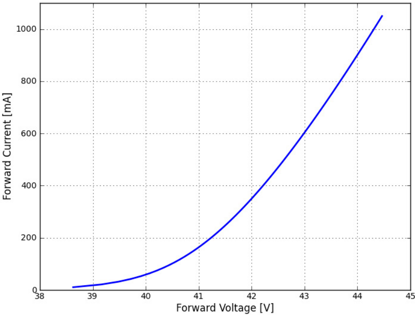
Figure 17. Forward current vs. forward voltage for LXXKx-Pxxx-xx16(A) products.
