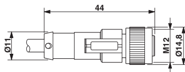
Dimensioned drawing
