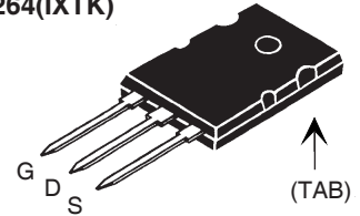
TO-264(IXTK)
