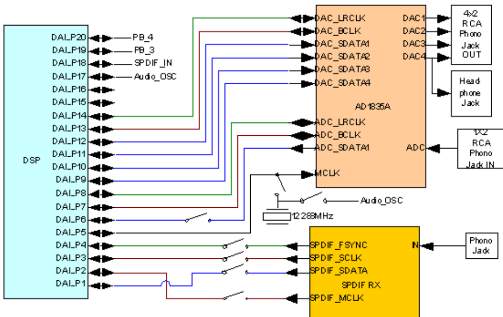
Figure 2-3. DAI Connections Block Diagram
