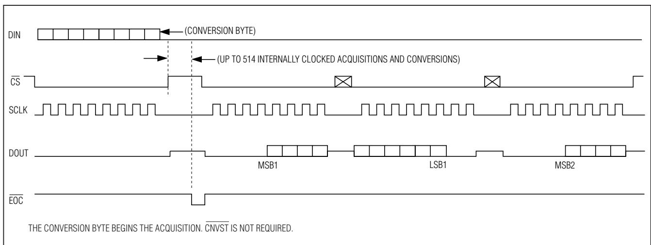
Figure 6. Clock Mode 10
