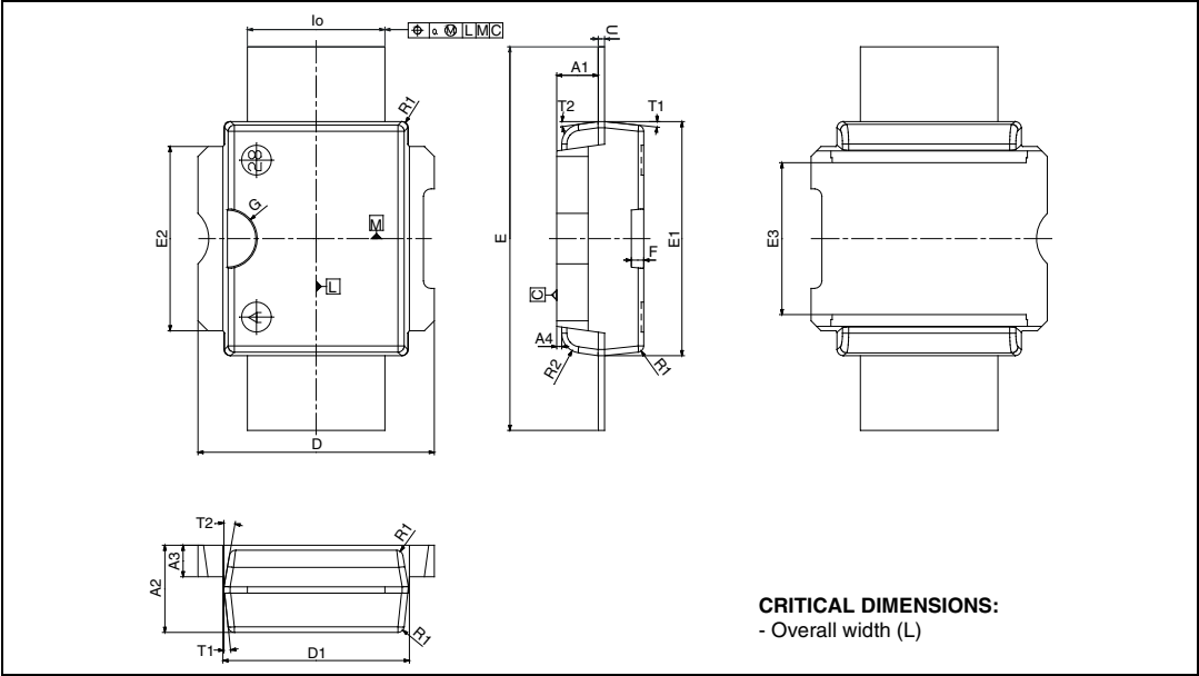
Figure 15. Package dimensions
