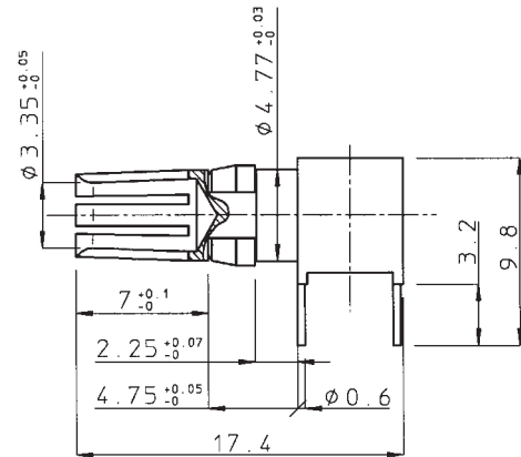
socket contact
