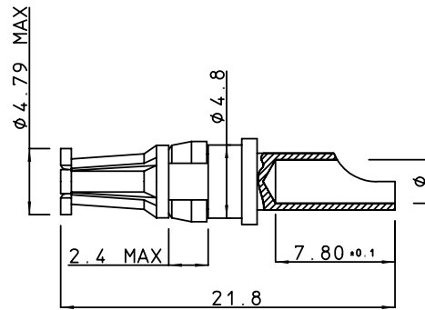
socket contact
