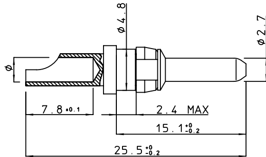
pin contact
