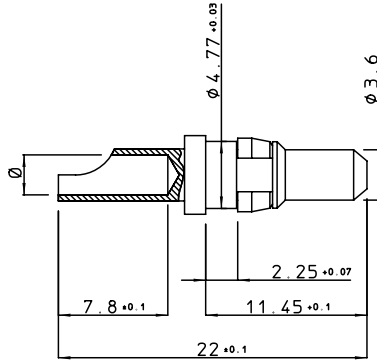
pin contact
