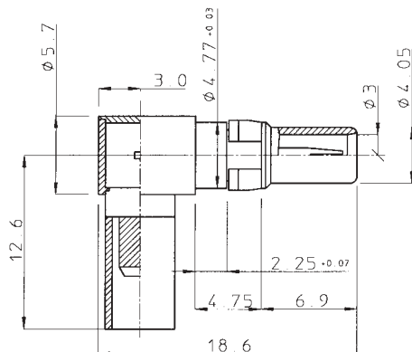
socket contact
