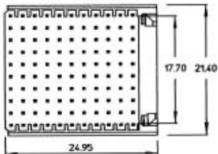
Standard loading patterns (seen from mating side)
