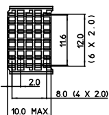
HM2H06P1□□ (type 5X5)
