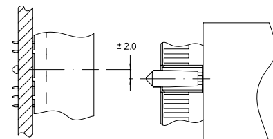
Allowed misalignment
