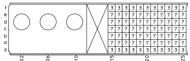
HM2P11PK5111GF
