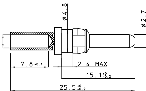
pin contact
