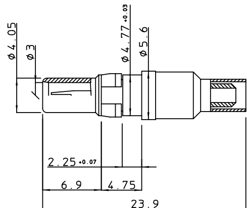
socket contact
