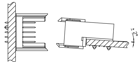
Allowed misalignment
