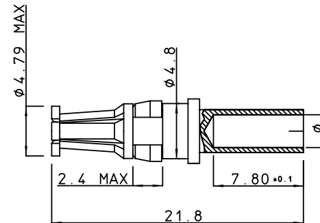
socket contact
