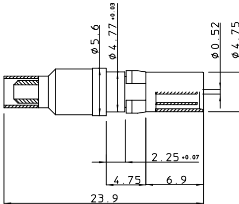
pin contact
