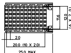
HM2H09P1□□ (type C)
