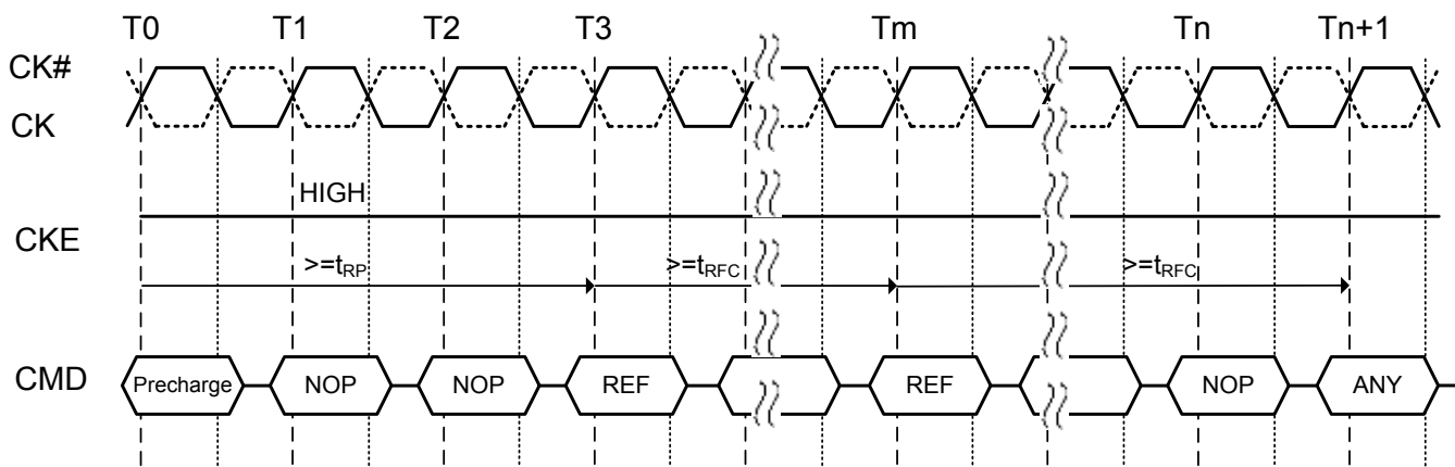
Figure 43. Refresh command
